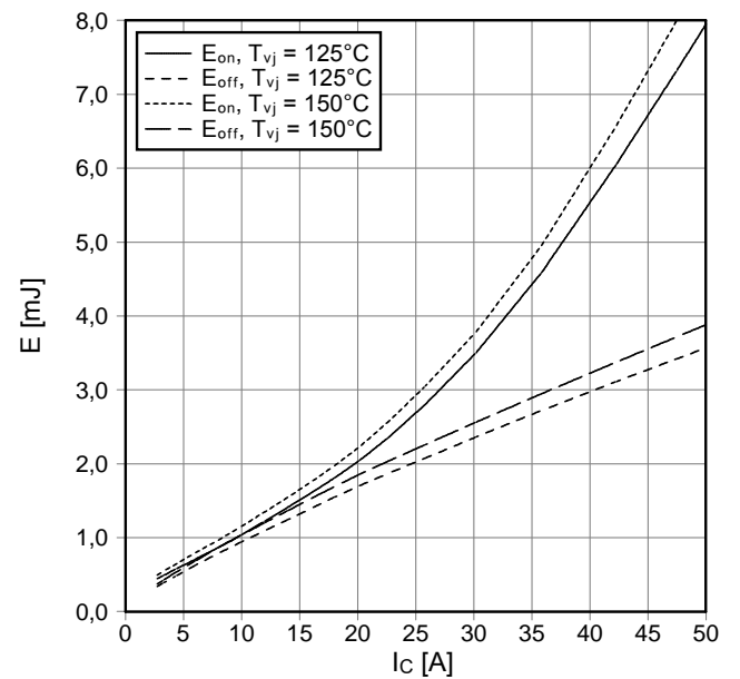
Schaltverluste IGBT-Wechselr. (typisch) switching losses IGBT-inverter (typical) E_{on} = f(I_C) , E_{off} = f(I_C) V_{GE} = \pm 15\text{ V} , R_{Gon} = 20\ \Omega , R_{Goff} = 20\ \Omega , V_{CE} = 600\text{ V}
